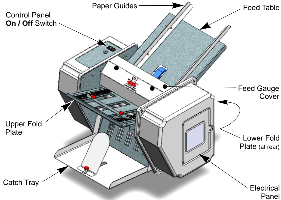
Figure 6: SPIRIT Diagram
