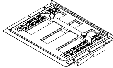
Figure 1: Upper Fold Plate
